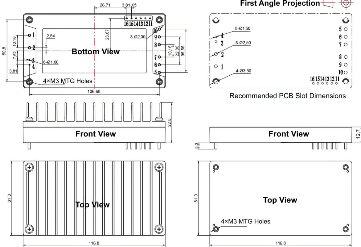
Standard + Heat sink 116.8*61.0*32.50mm
